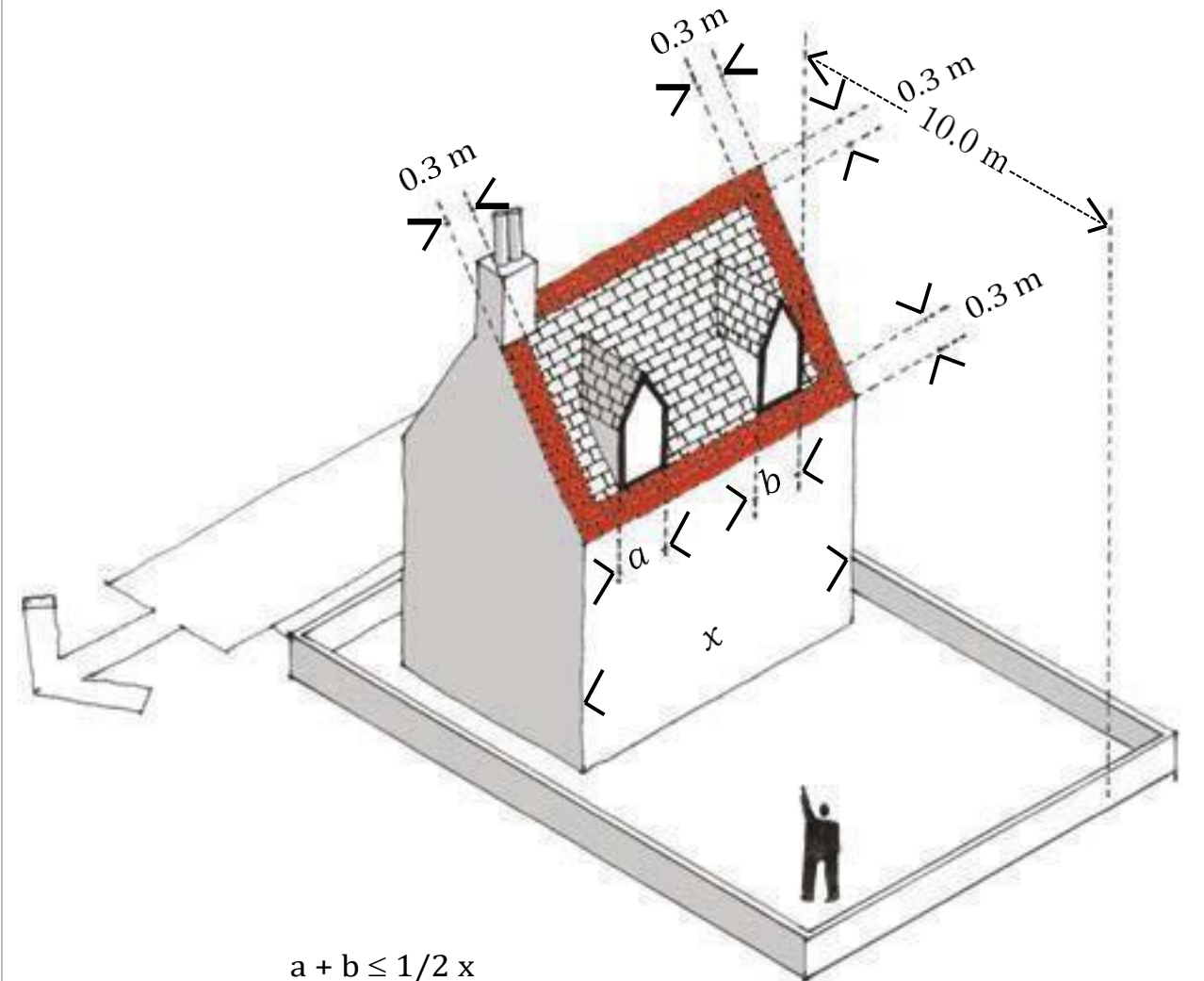
Figure 15: Roof enlargements
